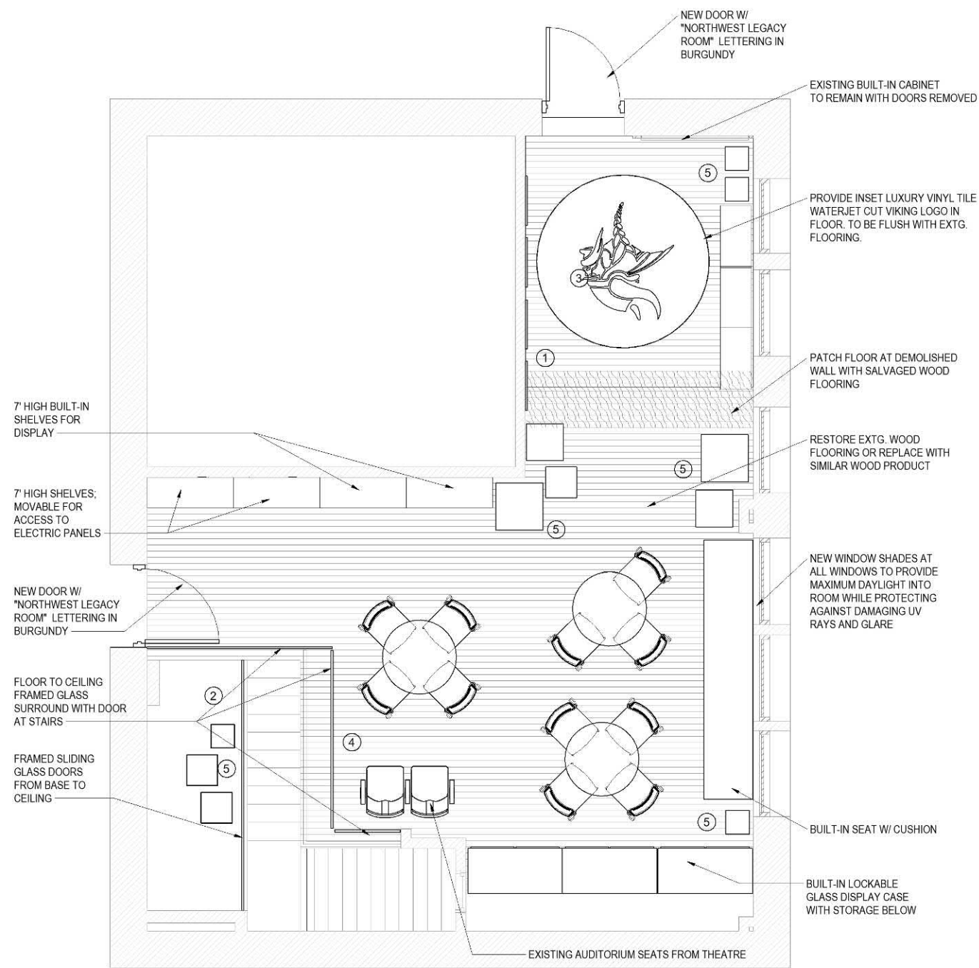
1 FLOOR PLAN SCALE: 3/8" = 1'-0"
